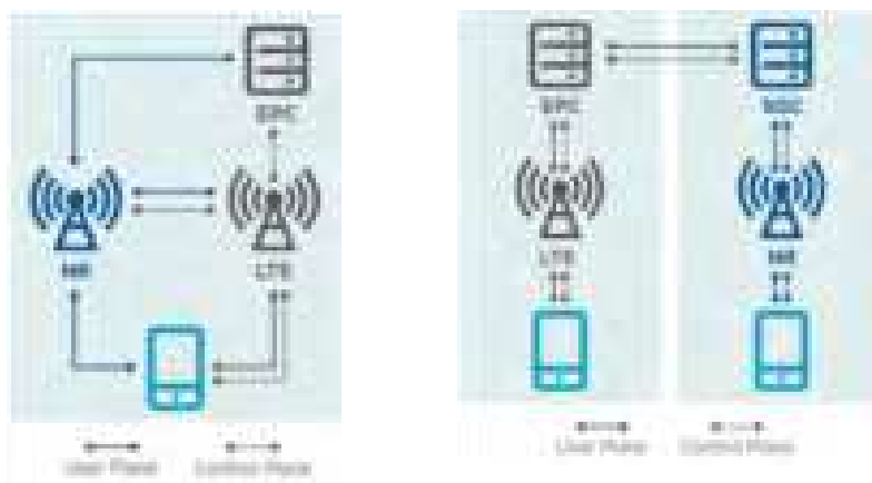
NON-STANDALONE (NSA) DEPLOYMENT STANDALONE (SA) DEPLOYMENT
